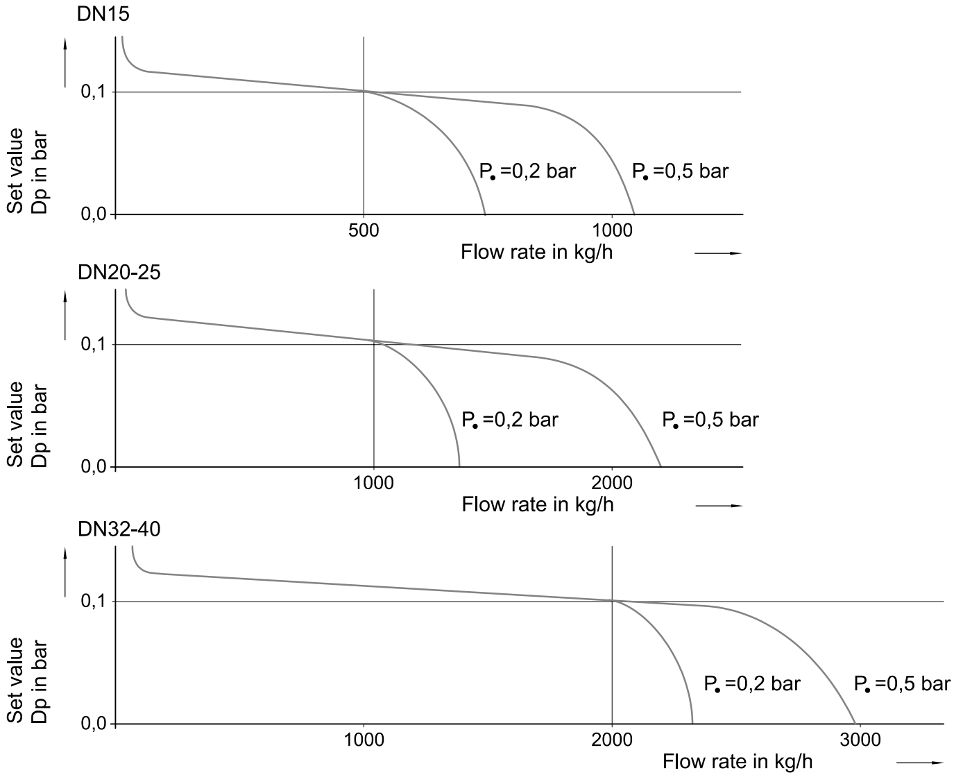
Fig. 4. Control characteristic of V5012C0103, set at 0.1 bar Dp (factory setting)
