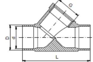
Anschweißenden ISO 4200 "L" / welded connection ISO 4200 "L"
